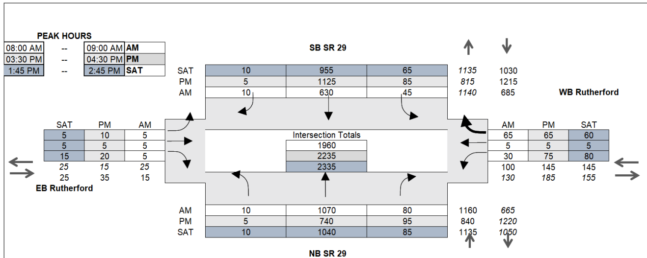
Figure 6.3 – Year 2035 Turning Movement Volumes – Rutherford Cross Road Intersection
