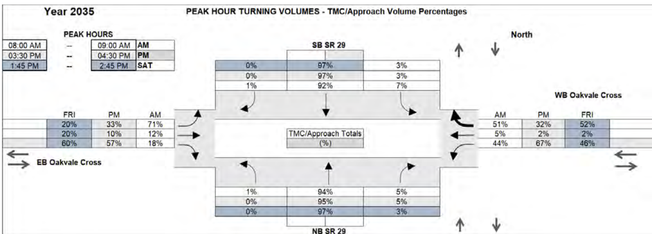
Figure 6.2 – Year 2035 Turning Movement Volumes in % of approach volumes– Oakville Cross Road Intersection
